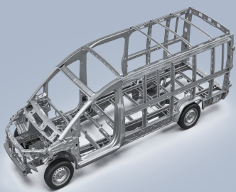
High-strength steel cage-type body structure
