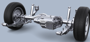
The design of an integrated rear axle
